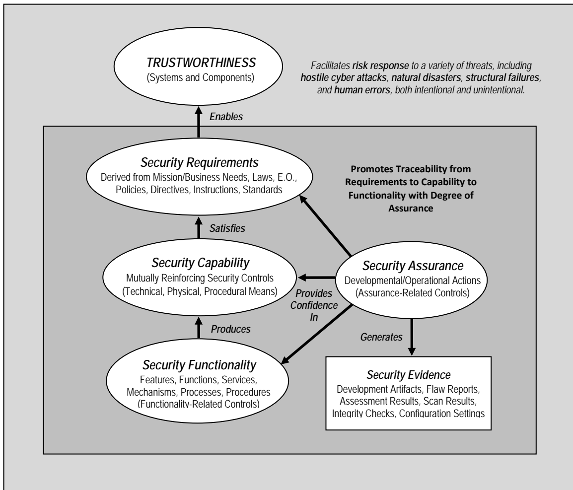
FIGURE 3: TRUSTWORTHINESS MODEL
